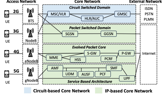
Figure 1: Cellular network architectures from 2G to 5G.
