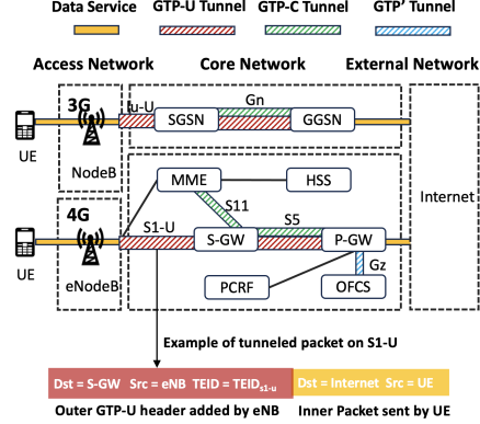
Figure 3: GTP tunnels in 3G and 4G core networks.
